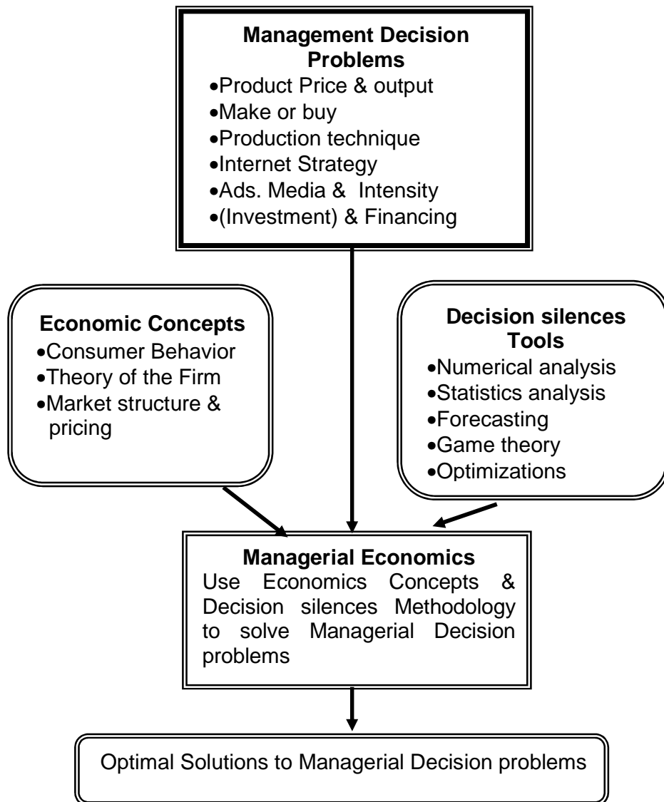
Figure 1.1: Decision-making model
