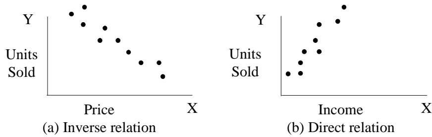
Figure 2.4: Scatter diagrams
