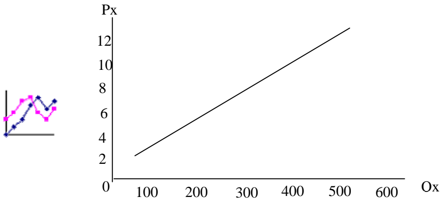
Figure 2.2: Supply curve
