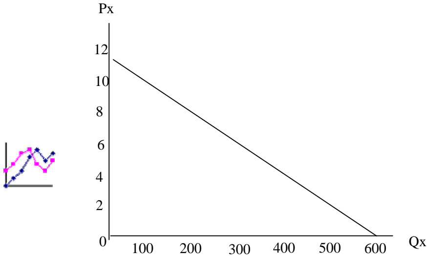
Figure 2.1: Demand curve
