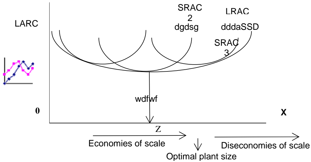
Figure 3.2: Long-run cost
